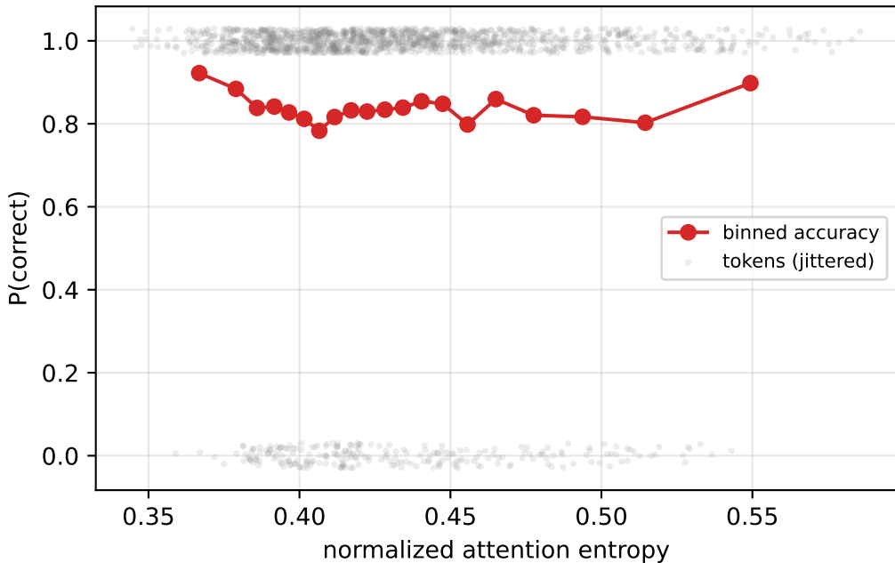
Entropy predicts errors (mixed) Pearson r=-0.021 , Spearman \rho=-0.020
