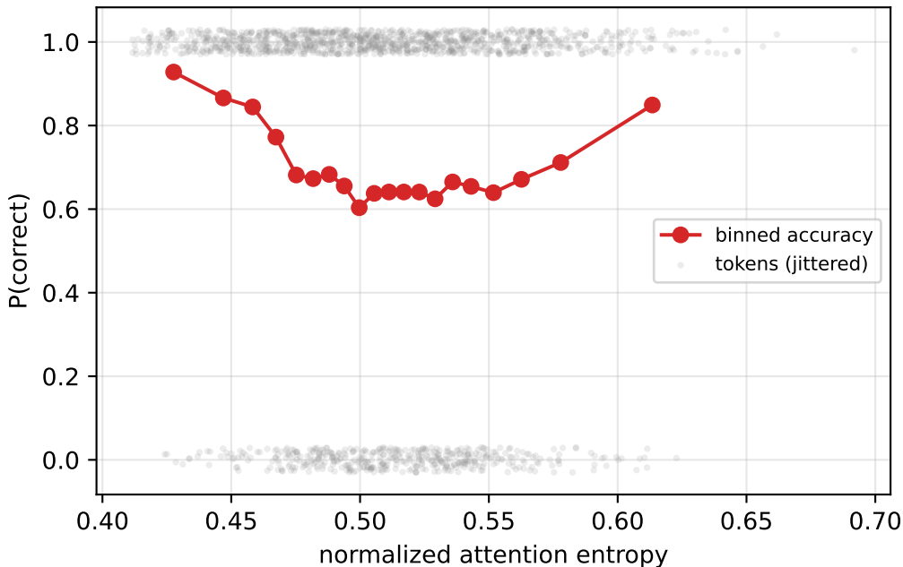
Entropy predicts errors (tagged) Pearson r=-0.012 , Spearman \rho=-0.035
