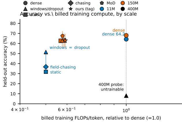
Figure 3: Accuracy vs. billed training compute (relative to the dense arm at the same scale, log axis; marker = arm, color = scale, values in Tables 1 and 2). Gated 2-stage arms cluster at \sim 0.58\times dense compute and \sim 5 points below it at 150M; MoD reaches dense compute savings with an inverted router. The 400M probe collapses (post-LN + Xavier init, untrainable at any LR swept), the honest edge of the scaling evidence; 1B was never run.
