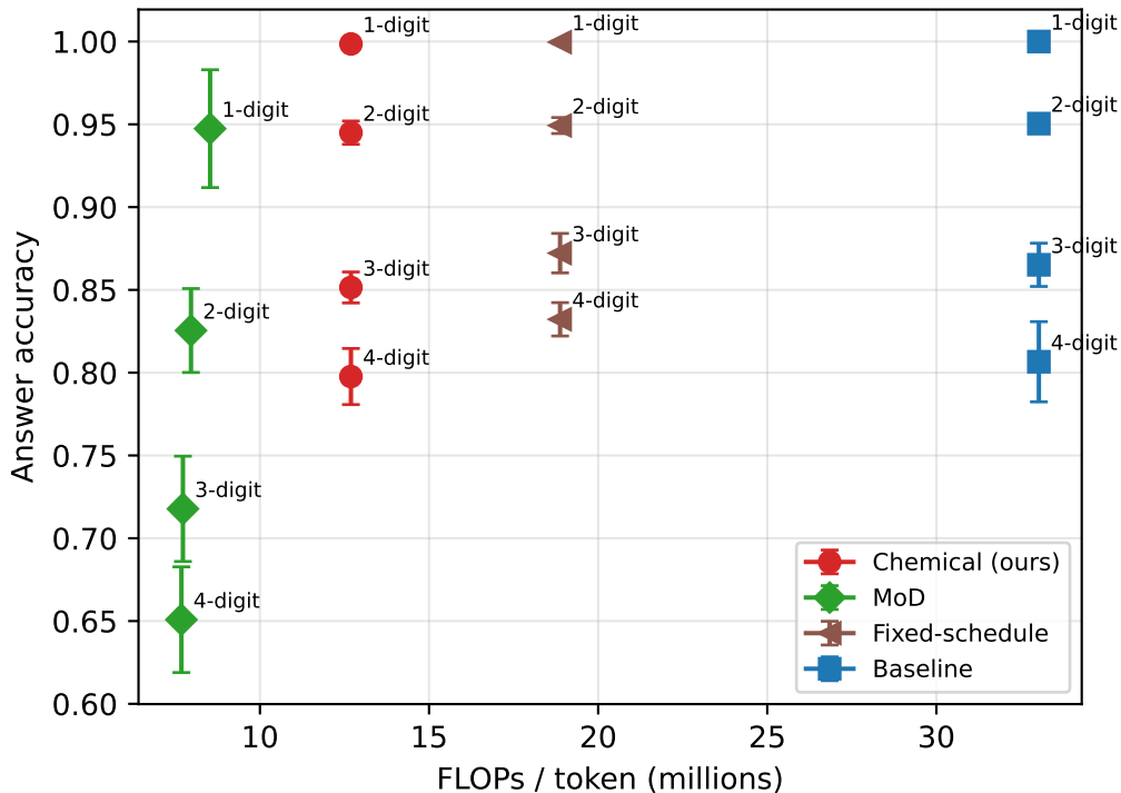
Accuracy vs. compute by difficulty (mixed)
