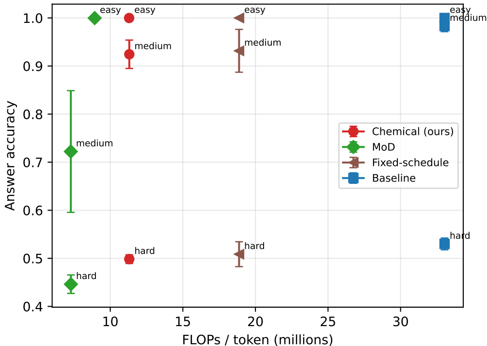
Accuracy vs. compute by difficulty (tagged)
