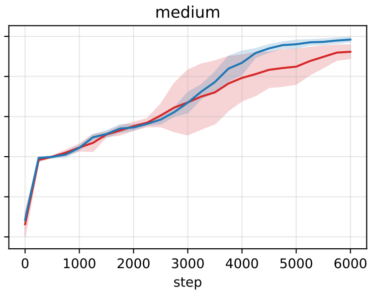
Per-difficulty accuracy over training (tagged)
