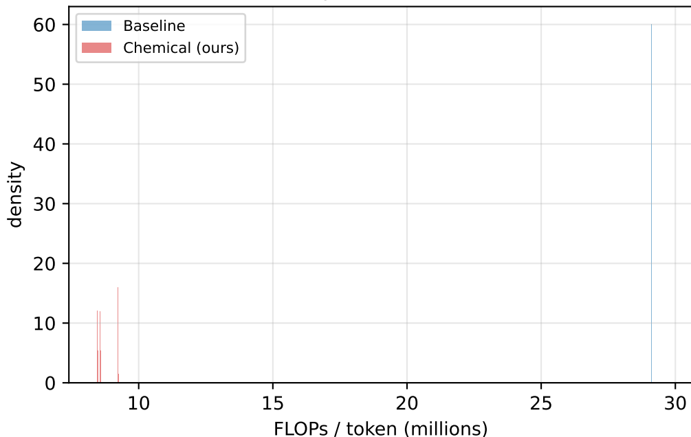
Per-token compute distribution (mixed)
