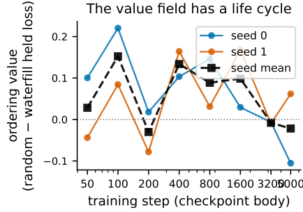
Figure 1: The life cycle, measured. Ordering value (random – waterfill held-out loss under zero-shot allocation on frozen checkpoint bodies; two seeds plus their mean) peaks at 0.1–0.2 over steps 100–800 and decays to zero by step 3200. The step-5000 sign flips are seed-inconsistent and pre-registered as noise, not claimed.
