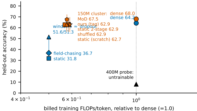
Accuracy vs. billed training compute, by scale ● dense ◆ field-chasing ⬠ MoD ● 150M ▲ dropout / windows ★ ours (tag) ● 11M ● 400M ■ static
