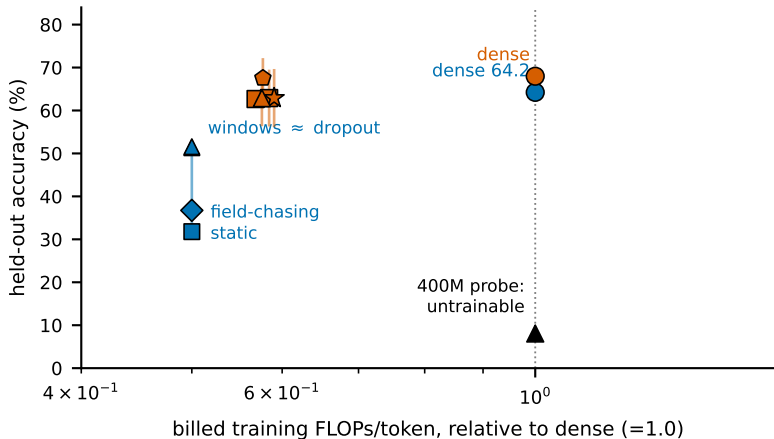
Accuracy vs. billed training compute, by scale ● dense ◆ chasing ⬠ MoD ● 150M ▲ windows/dropout ★ ours (tag) ● 11M ● 400M ■ static
