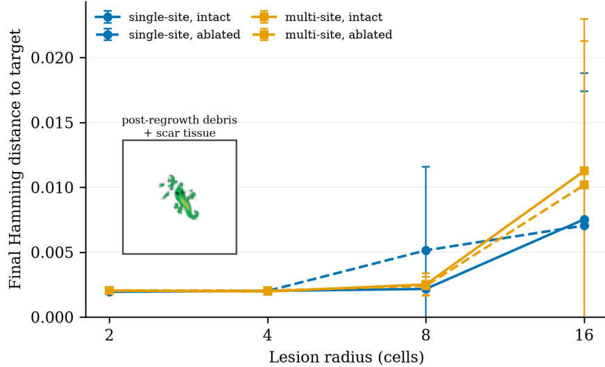
Figure 1: E1 lesion sweep. Final Hamming distance as a function of lesion radius and kind, with and without modulator channels (mean \pm SD over 5 damage seeds). Inset: post-regrowth debris and scar tissue.
