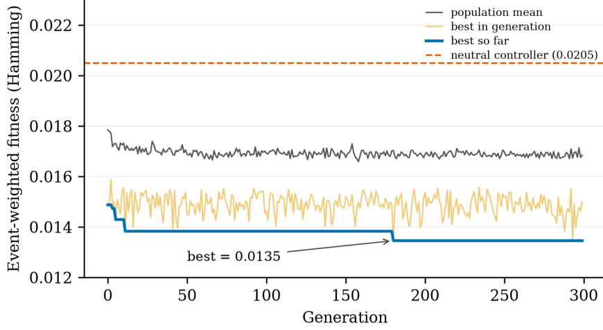
Figure 2: CMA-ES fitness over 300 generations ( \sigma_0=0.01 ). Dashed line: neutral controller (0.0205). Best evolved fitness: 0.0135 — a 34% improvement with no stall.
