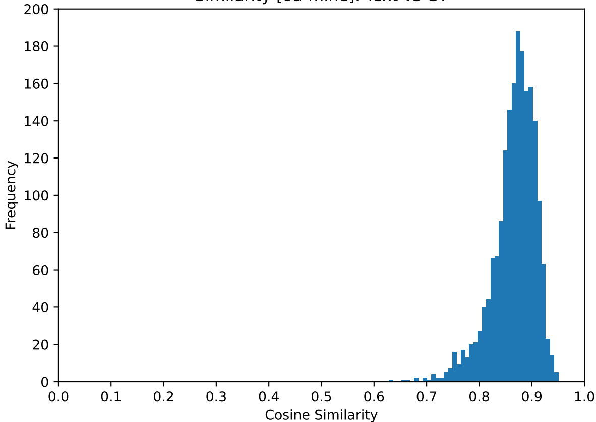
Similarity [oa-mine]: Text vs GT
