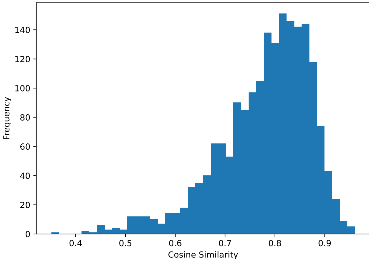
Similarity [mave]: Text vs LX
