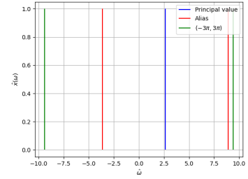
Figure 10.20: Spectrum of x(t) , we see 3 spectral components in the range (-3\pi, 3\pi)
