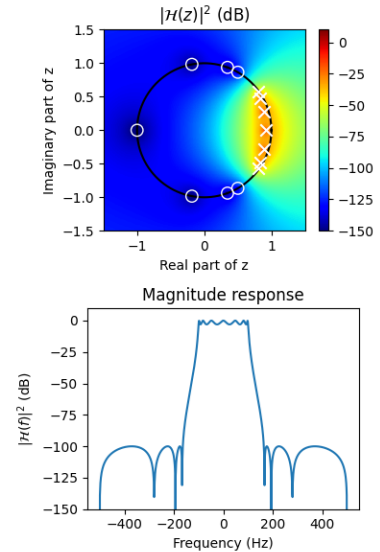
Figure 22.12: The pole-zero diagram and magnitude response of the designed IIR low-pass filter. The bandwidth is specified to be 100 Hz, with the stop-band starting at 200 Hz. Spectral components of the signal in the stop-band are attenuated by at least 100 dB.
