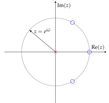
Figure 21.13: Locations of the three zeros ( \alpha_k = \{e^{i\frac{\pi}{3}}, e^{-i\frac{\pi}{3}}, 1\} ) of \mathcal{H}(z) in the complex plane are marked with blue circles. In this case, they all coincide with the unit circle.
