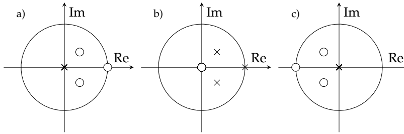
Figure 22.14: Three different pole-zero diagrams. The unit circle z = e^{j\hat{\omega}} is marked in each diagram with a solid black line. The zeros of the system function \mathcal{H}(z) are marked with circles (o) and the locations of the poles are marked with crosses (x). The real and imaginary components of poles and zeros only consist of the following numbers: 0, \pm 1 , or \pm(2\sqrt{2})^{-1} .
