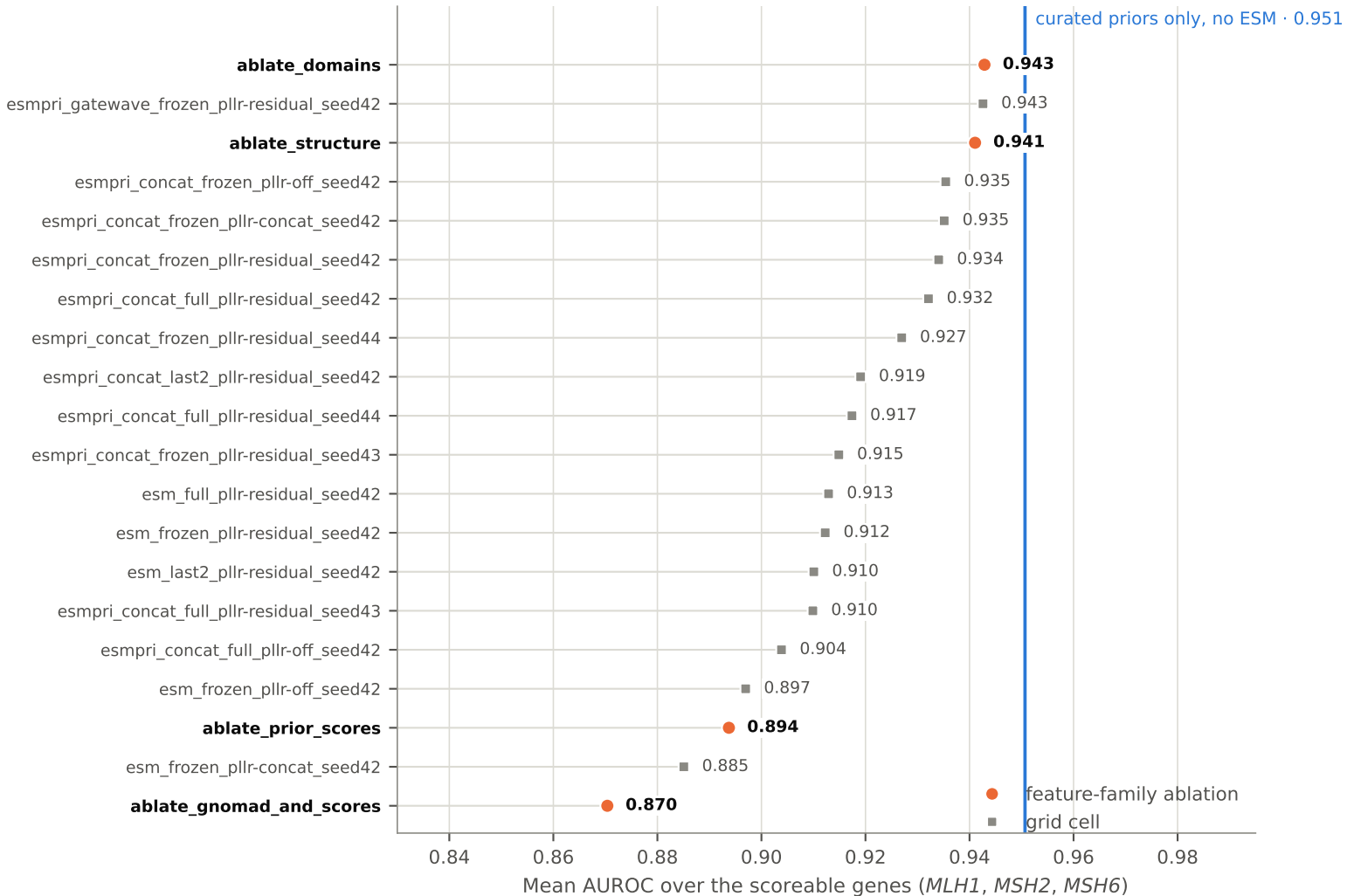
Ablation grid and feature-family removals, ranked
