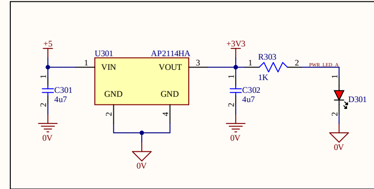
POWER REGULATOR (+5V to +3V3)
