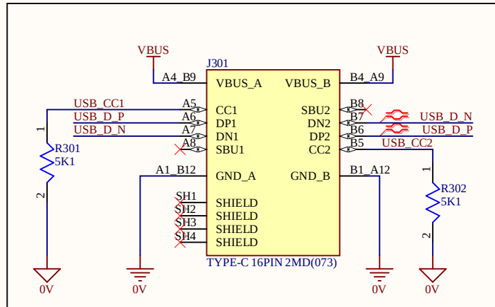
TYPE-C USB SOCKET
