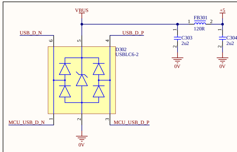
ESD PROTECTION + PI FILTER
