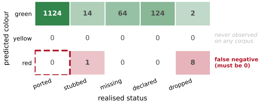
(a) all corpora, 1337 items
