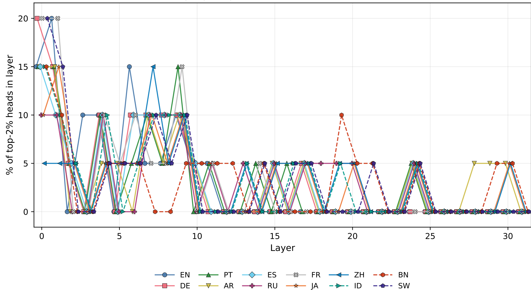
Where language-important heads cluster — OLMo-2-7B (SFT)
