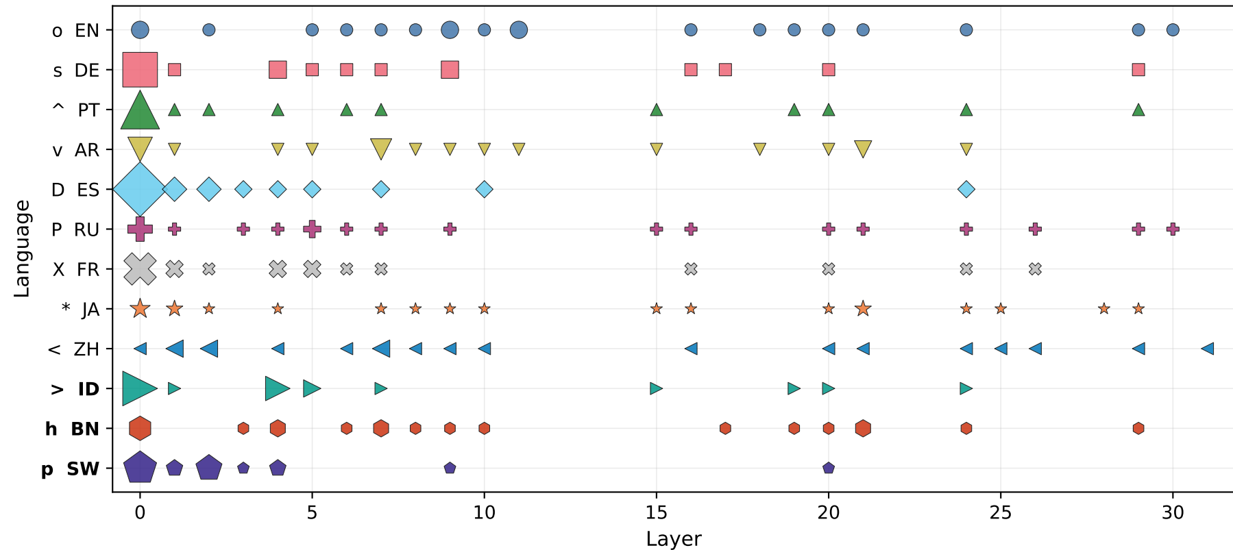
Where language-important heads cluster — OLMo-2-7B (base) (marker area = % of that language's top-2% heads; no marker = 0%; bold = low-resource)
