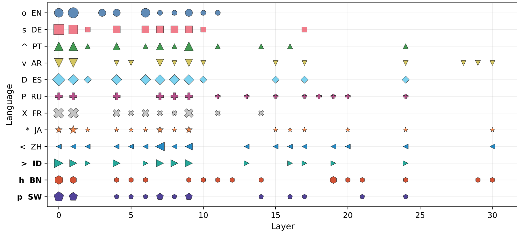
Where language-important heads cluster — OLMo-2-7B (SFT) (marker area = % of that language's top-2% heads; no marker = 0%; bold = low-resource)
