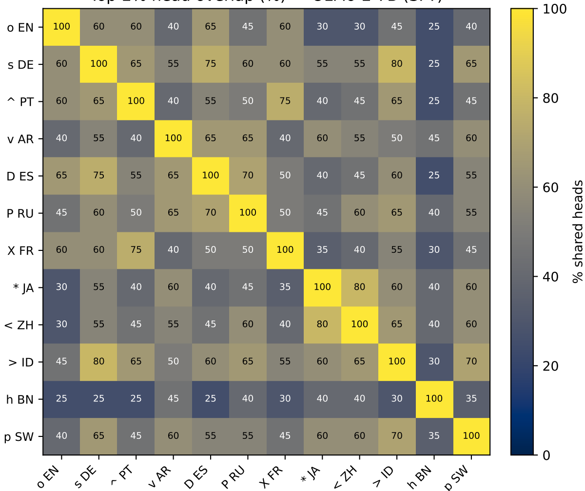
Top-2% head overlap (%) — OLMo-2-7B (SFT)
