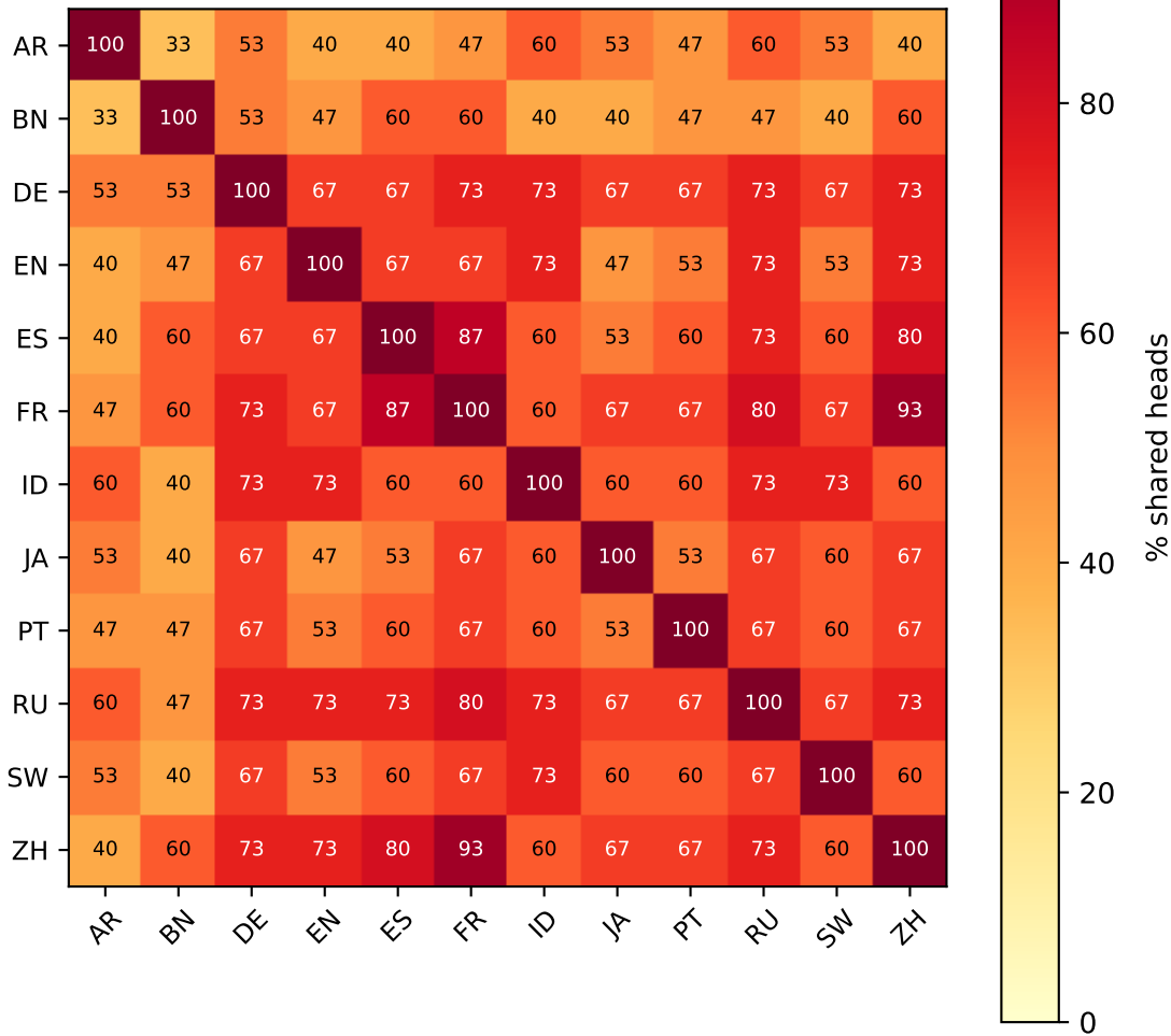
Head Overlap — Qwen-2.5-7B (SFT)
