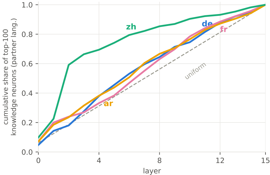
fair tokenizer
