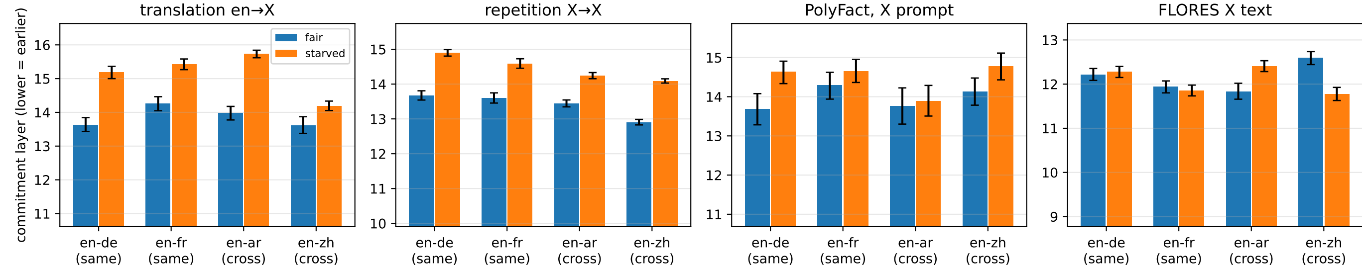
Layer from which the lens settles on the final answer, by task and partner
