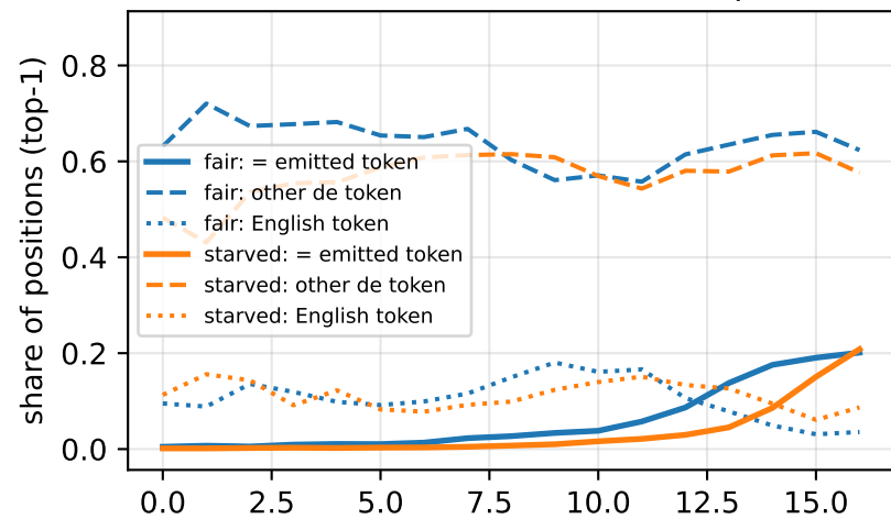
en-de: de text, lexical word-initial positions
