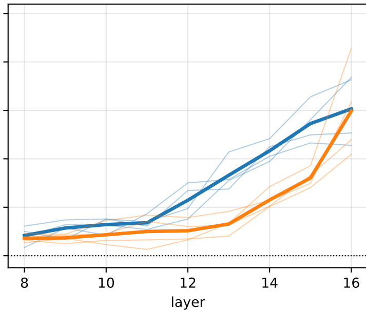
matched partner-language BPB
