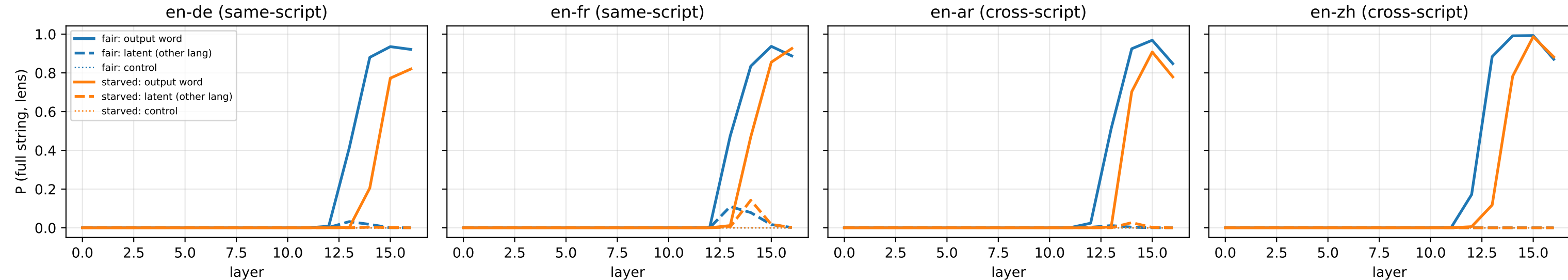
repetition X→X: probability of output word vs its other-language translation, by layer
