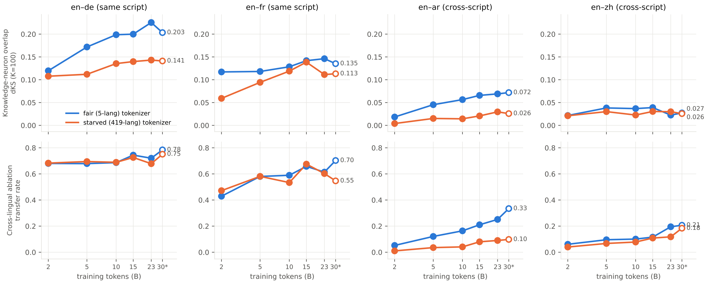
Parametric knowledge sharing over training (* 30B = cooled final; 2-23B mid-stable at peak LR; hollow marker = cooled)
