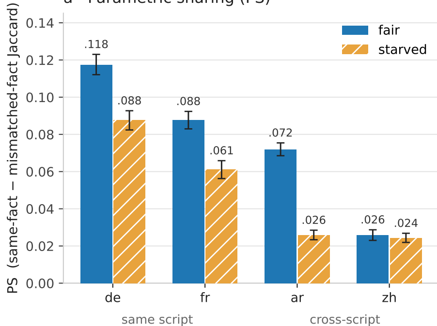
a Parametric sharing (PS)
