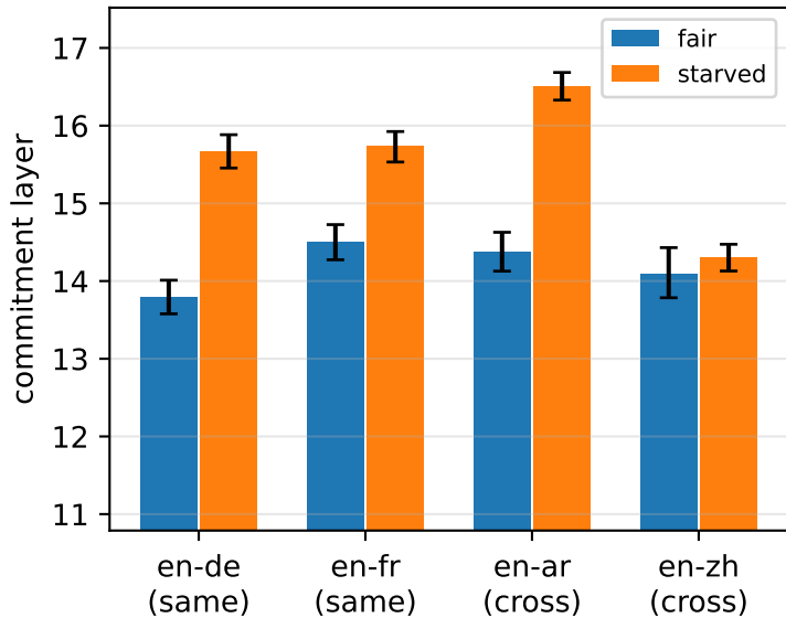
translation en→X
