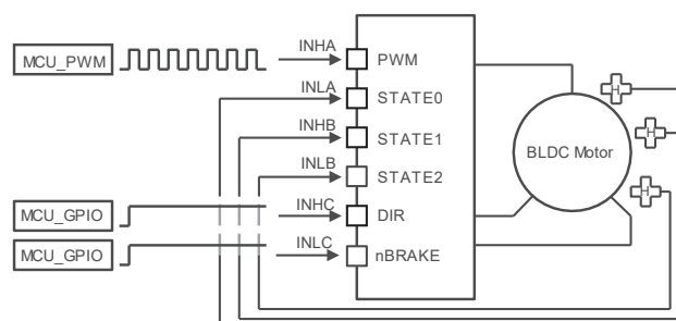
Figure 19. 1x PWM—Hall Effect Sensor
