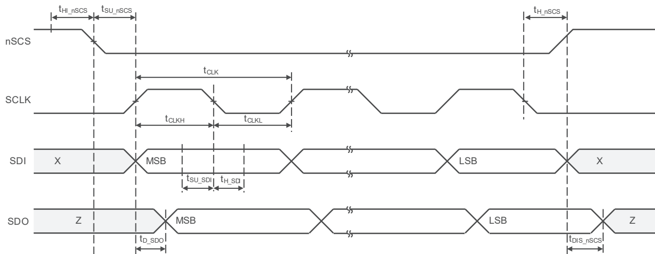
Figure 1. SPI Slave Mode Timing Diagram
