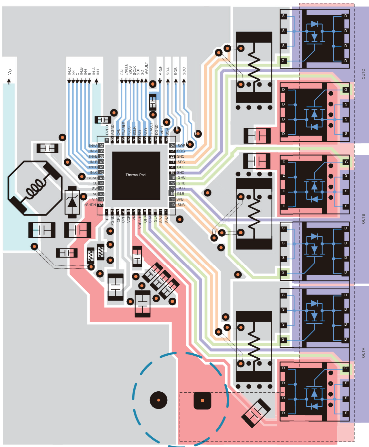
Figure 66. Layout Example
