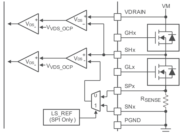
Figure 29. DRV8323 and DRV8323R V_{DS} Monitors
