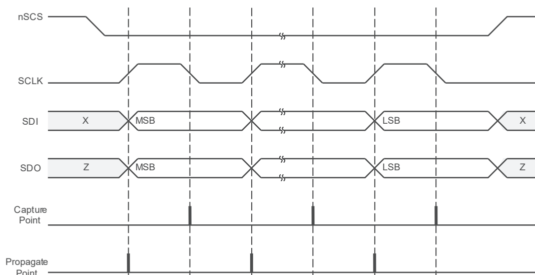
Figure 45. SPI Slave Timing Diagram
