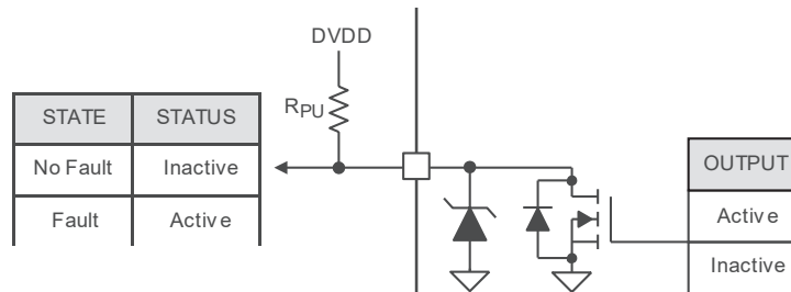
Figure 34. Open-Drain Output Pin Structure
