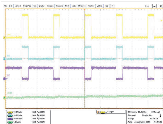
Figure 54. Gate Drive at 20% Duty Cycle
