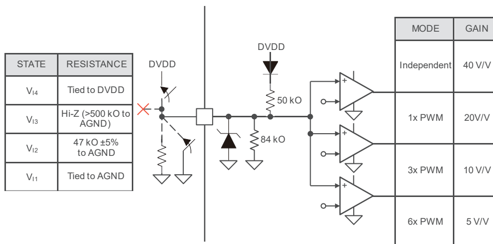
Figure 32. Four Level Input Pin Structure
