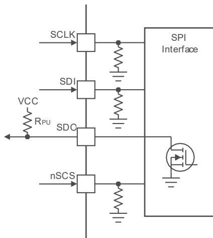
Figure 23. SPI
