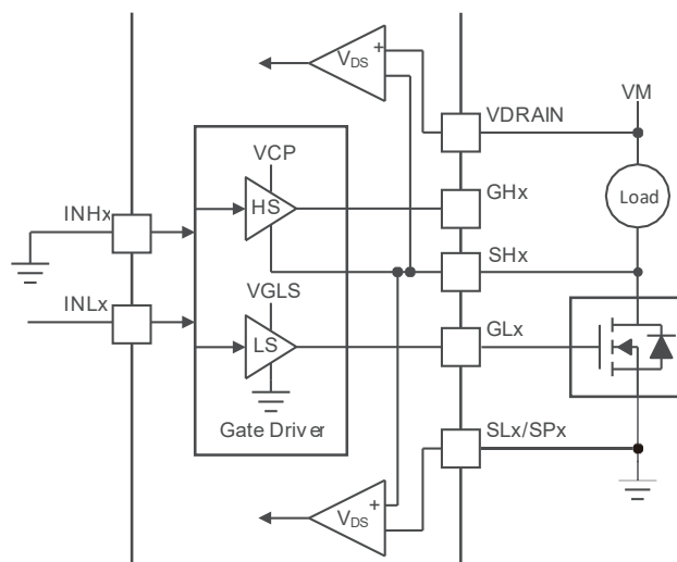
Figure 22. One Low-Side Driver
