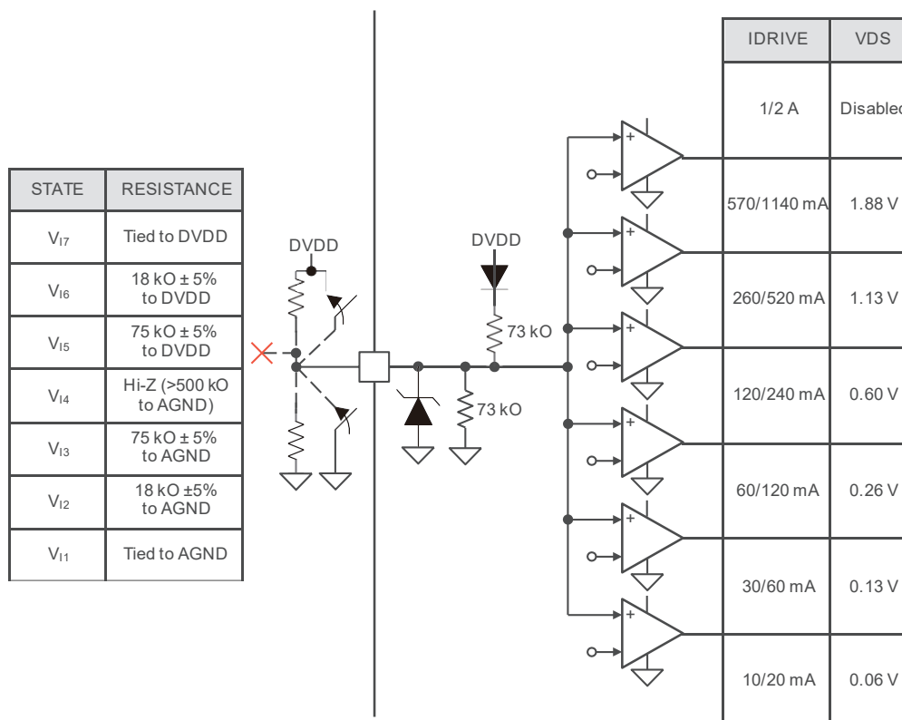
Figure 33. Seven Level Input Pin Structure
