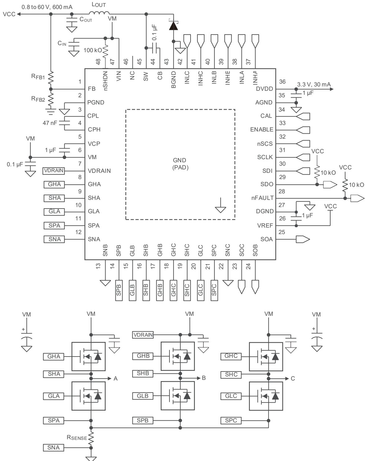
Figure 64. Alternative Application Schematic
