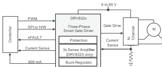
Simplified Schematic
