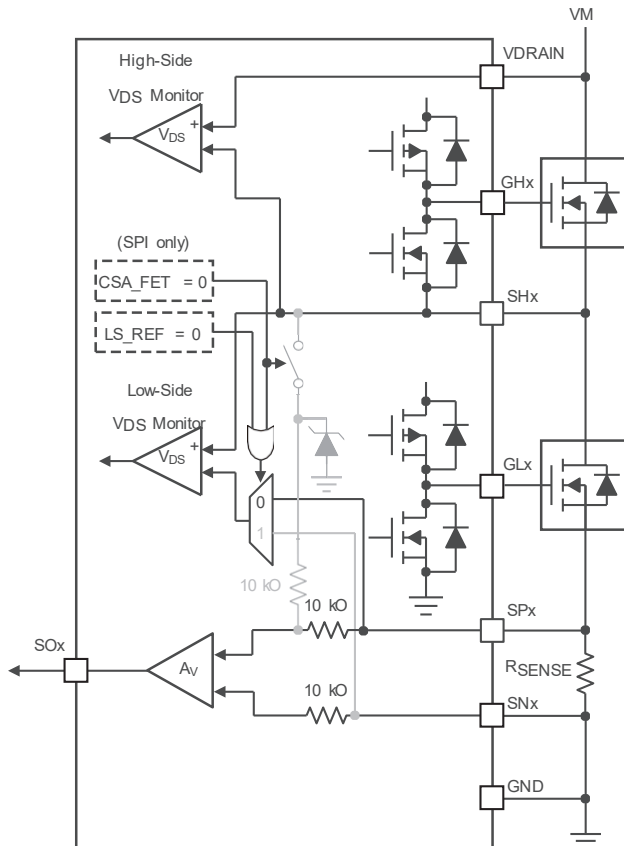
Figure 41. Resistor Sense Configuration
