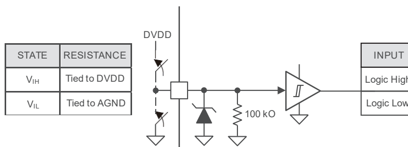
Figure 31. Logic-Level Input Pin Structure
