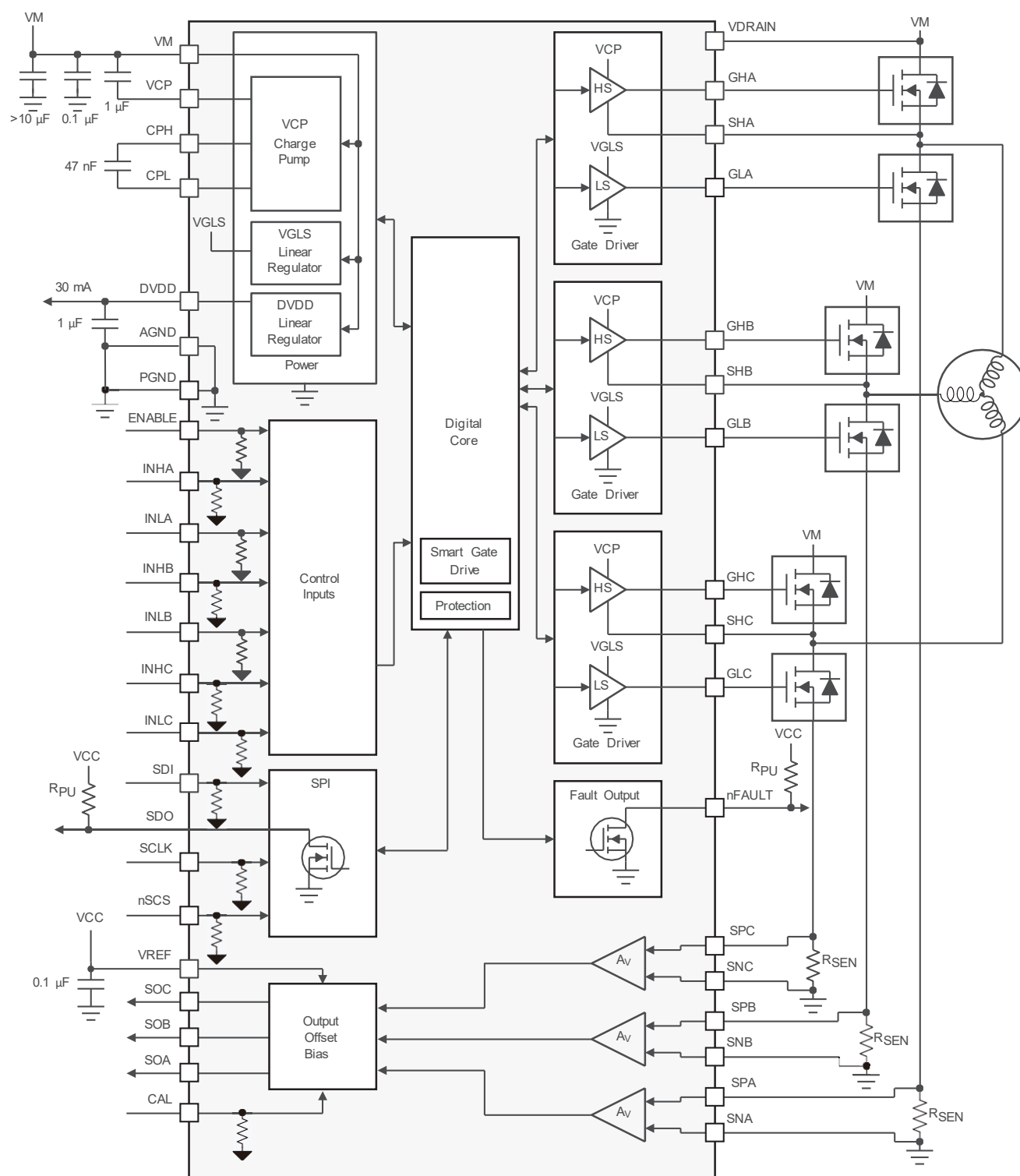
Figure 15. Block Diagram for DRV8323S
