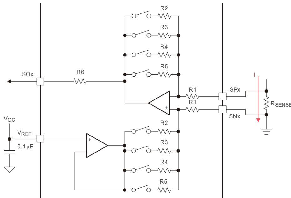
Figure 38. Unidirectional Current-Sense Configuration
