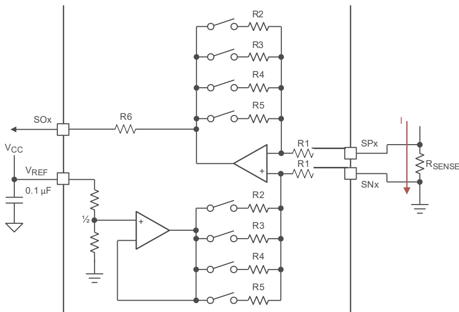
Figure 35. Bidirectional Current Sense Configuration
