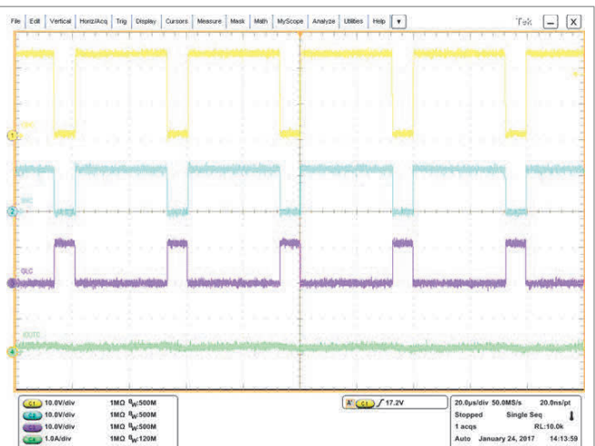
Figure 55. Gate Drive at 80% Duty Cycle
