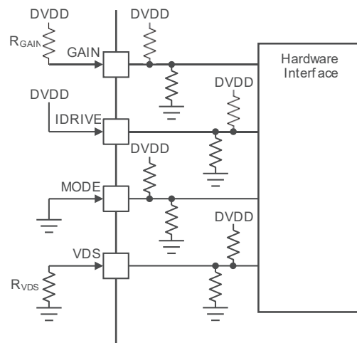
Figure 24. Hardware Interface
