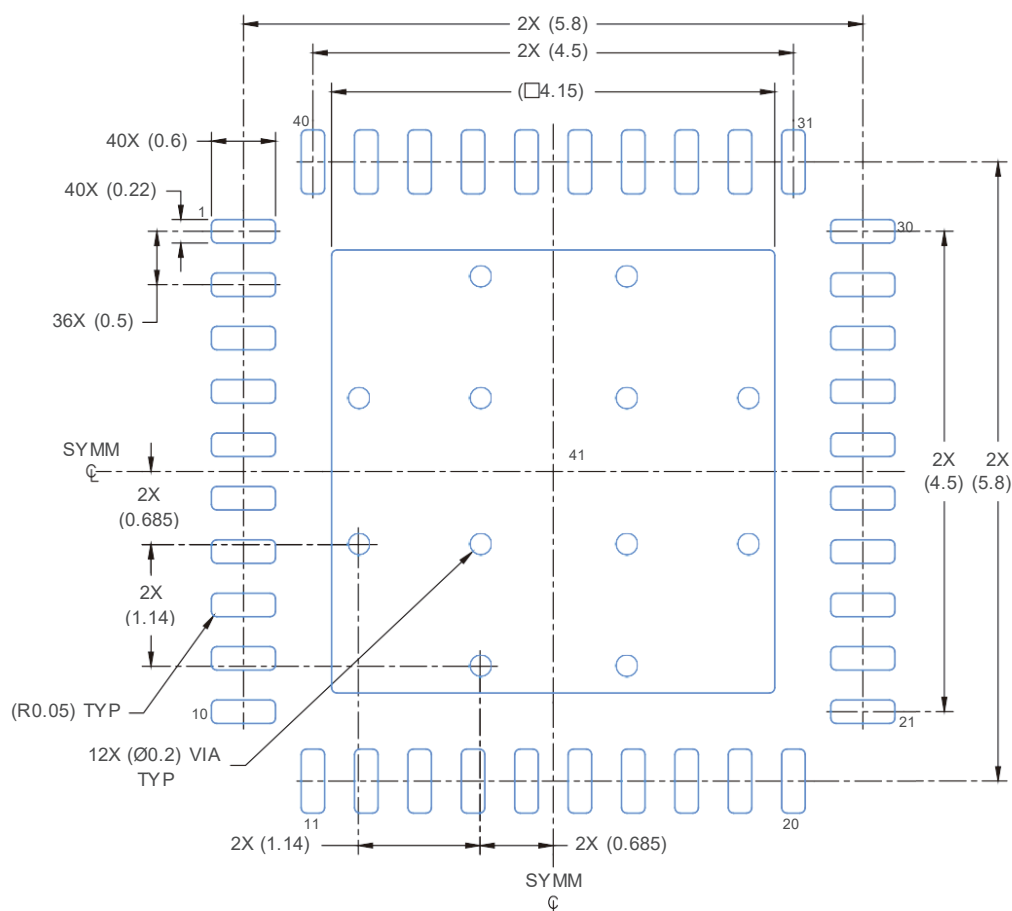
LAND PATTERN EXAMPLE
