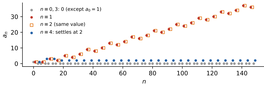
FIGURE 1. The first 150 terms of the sequence started from 1, 1, 1, 0, 1, 0, 1, 1, coloured by the remainder of n on division by 5. Positions with remainder 0 or 3 hold 0 (apart from a_0 = 1 ), positions with remainder 4 settle at 2, and the twin positions with remainders 1 and 2 carry equal values that grow by 4 every three blocks.
