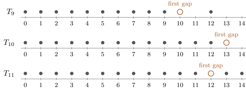
FIGURE 4. The first gap moves through 10, 13, 12 in three consecutive blocks. Filled dots are numbers present in the set; the open circle is its mex. The proof below explains why the same pattern returns four units farther along.
