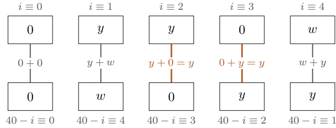
FIGURE 2. The pairs (i, 40 - i) that determine a_{41} , grouped by remainders modulo 5. The boxes show the usual values: 0, a twin value y , or a last-column value w . In the first pairing there is one exception: position 0 holds 1, so (0, 40) and its reverse contribute 1. The two highlighted pairings copy every earlier twin value.
