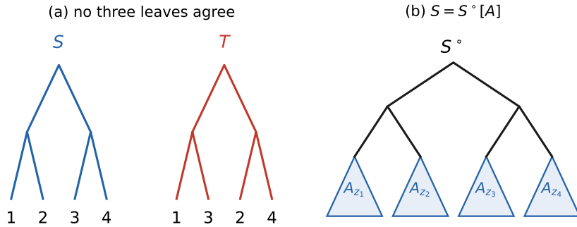
FIGURE 1. (a) Two balanced trees on four leaves whose largest agreement subtree has two leaves. (b) The substitution S^\circ[A] of Section 3: each leaf z of S^\circ becomes the root of a tree A_z . An agreement set of S^\circ[A] and T^\circ[B] can use at most \text{mast}(S^\circ, T^\circ) of the blocks, and at most \text{mast}(A_z, B_z) leaves inside each.
