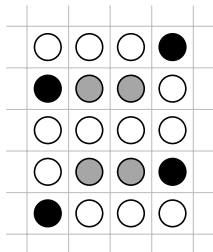
FIGURE 2. A finite arrangement for (a, b, c) = (1, 1, 6) : every A (white) touches one B (black), every B touches one C (grey), and every C touches six A 's.
