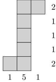
FIGURE 4. The heptomino A with its row counts P = (2, 1, 1, 1, 2) and column counts Q = (1, 5, 1) .
