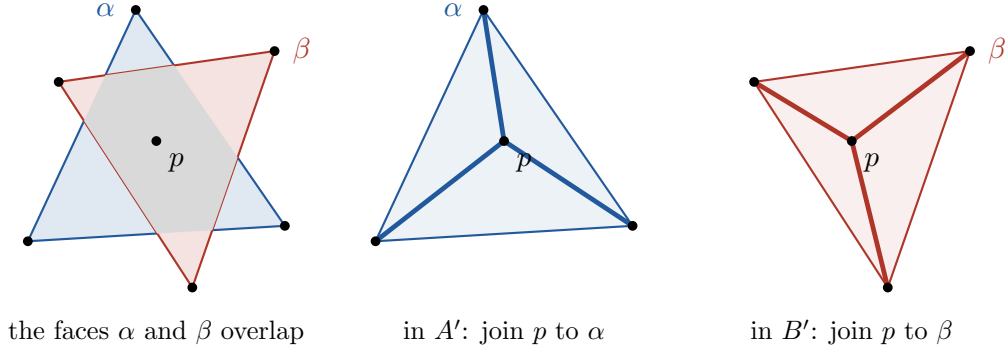
Figure 3. Lemma 6. The point p lies in the overlap of \alpha and \beta (shaded). The three thick blue edges are added to A and the three thick red edges to B .
