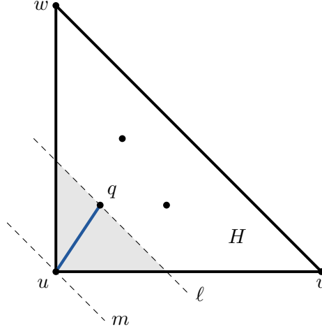
Figure 2. Lemma 3 for a triangular hull. The line m through u is parallel to vw ; q is the point nearest to it, and \ell is the parallel through q . The shaded strip between m and \ell contains no point of the set, so no segment crosses uq (thick).
