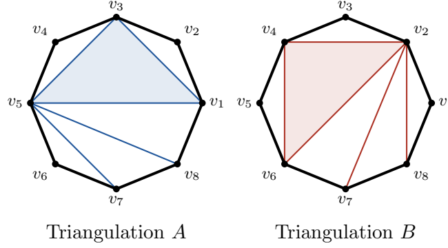
Figure 5. Lemma 9 for h = 8 . The side v_1v_3 of the shaded face v_1v_3v_5 of A passes through the faces v_2v_4v_6 (shaded) and v_2v_6v_7 of B . For h = 6 the fans are empty.
