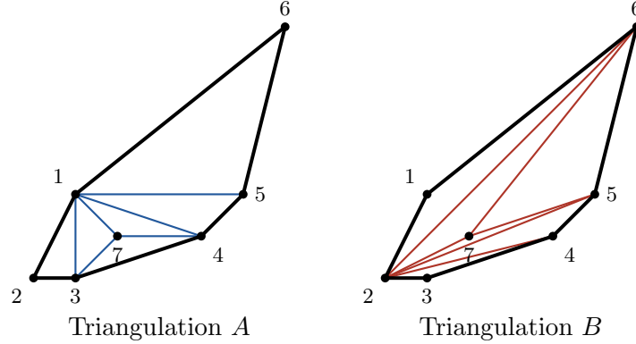
Figure 6. Two triangulations of seven points with a hexagonal hull, sharing only the six hull edges (black).
