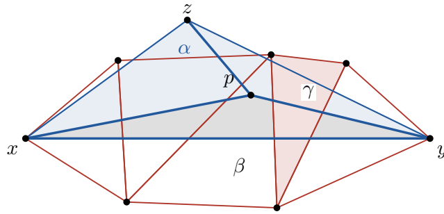
Figure 4. Lemma 8. The side xy of \alpha = xyz passes through the faces \beta and \gamma of B (red; faces of B away from xy are omitted, and \beta is drawn before it is subdivided). After p is inserted in \alpha \cap \beta , the face pxy of A' (grey), the face \gamma (shaded) and a piece of \beta form the next chain.
