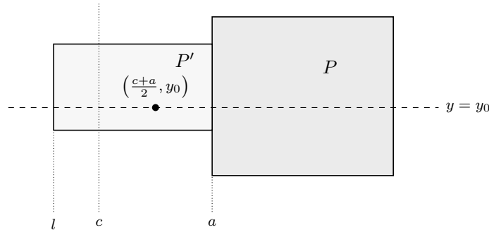
FIGURE 8. Lemma 8. The rectangle P' covering the point between c and a must end exactly at a ; otherwise it would overlap P along the line y = y_0 . Its left side l is an integer, so a is too.
