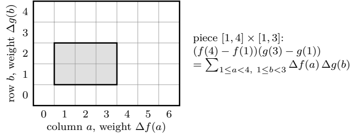
FIGURE 4. The proof of Lemma 2. Give the unit cell in column a and row b the weight \Delta f(a) \Delta g(b) . A piece's term is the total weight of its cells, and every cell lies in exactly one piece.
