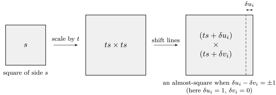
FIGURE 3. What a shift does to one square. After scaling, the cut lines around it move by small integers, changing its width by \delta u_i and its height by \delta v_i .
