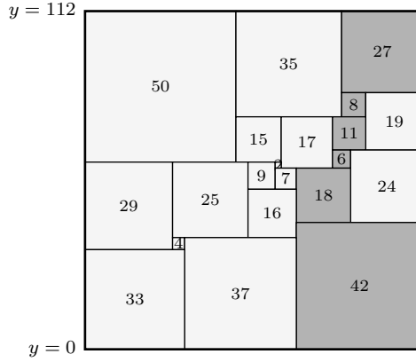
FIGURE 6. Six squares of Duijvestijn's square stacked from bottom to top. Each interior horizontal line between them is the top of one and the bottom of the next, and each of x = 70, 82, 85, 88, 93, 112 is a vertical side exactly twice. Only y = 0 and y = 112 occur once.
