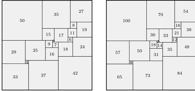
FIGURE 5. Duijvestijn's squared square of side 112 and its inflation at t = 2 , an admissible tiling of R_{224} by 21 almost-squares. Three vertical and six horizontal cut lines have moved, by at most two units.
