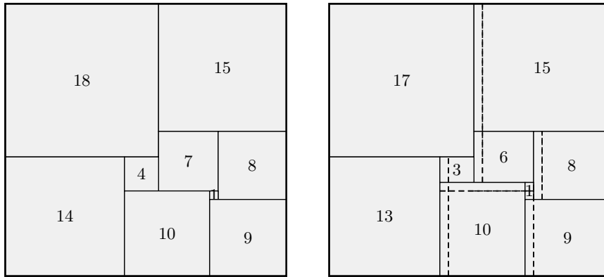
FIGURE 1. Left: Moron’s 33 \times 32 rectangle cut into nine distinct squares, labelled by side. Right: the vertical cut lines at x = 14, 18, 24, 25 move one unit left and the horizontal line at y = 10 moves one unit up (old positions dashed). Every square becomes an almost-square, labelled by size.
