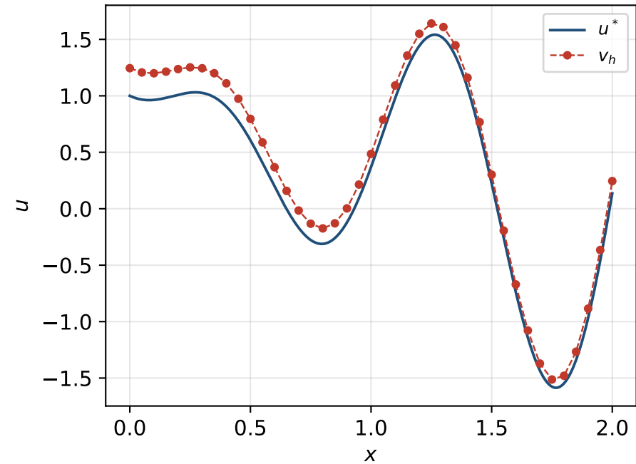
n = 40, O(h^1)
