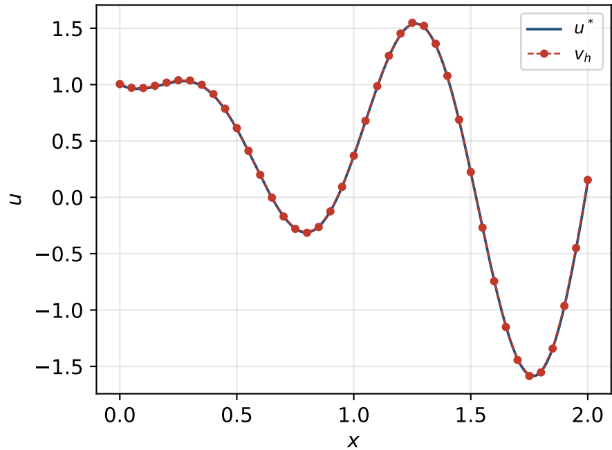
n = 40, O(h^2)
