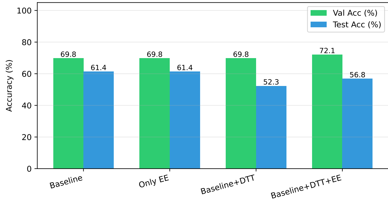
Ablation: Baseline vs +DTT vs +DTT+Early Exit
