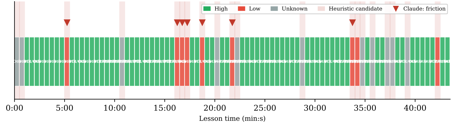
Strategy quality timeline — M-AU1 (20/87 heuristic candidates; 7 confirmed by Claude)
