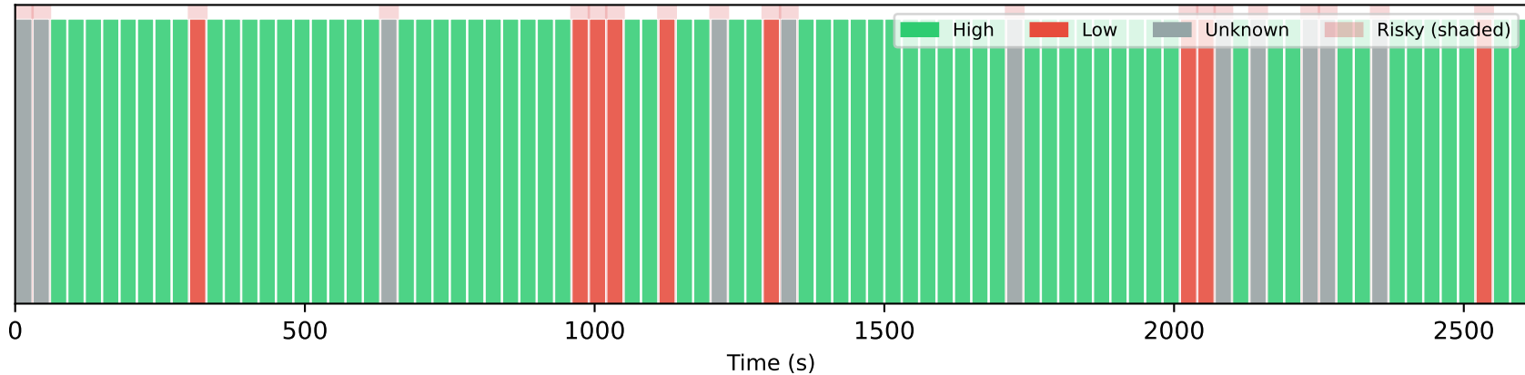
Strategy quality timeline — M-AU1 (20/87 bins flagged as risky)
