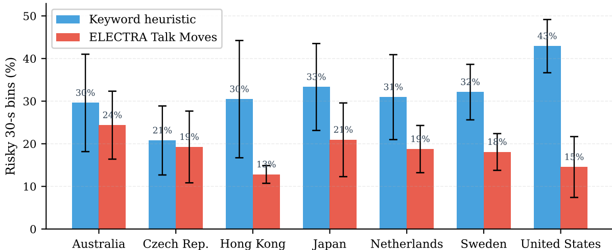
Keyword heuristic vs. ELECTRA Talk Moves (Pearson r = -0.35 , n = 53 lessons)
