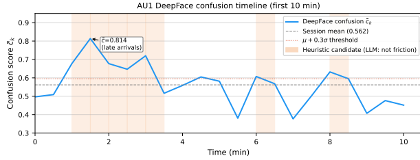
Figure 3: DeepFace confusion timeline for AU1 (10 min). Shaded regions are heuristic candidates; the peak ( \bar{C}_k=0.814 ) is caused by late-arriving students. LLM fusion rejects all 7 candidates.
