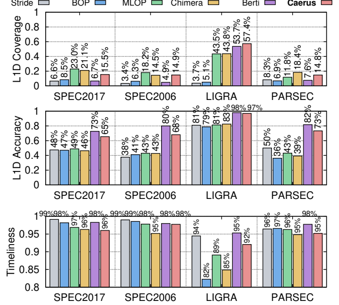
Fig. 14: Accuracy, Coverage and Timeliness.
