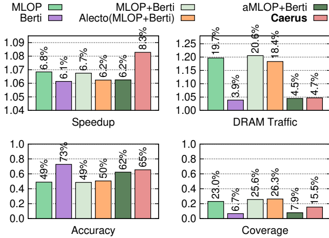
Fig. 16: Caerus compared with combinations of global and PC-local offset L1D Prefetchers in SPECspeed 2017.
