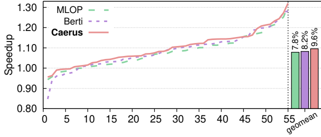
Fig. 18: Speedup of Caerus, MLOP, and Berti across 55 randomly selected 8-core heterogeneous workload mixes from all benchmark suites (sorted by speedup).
