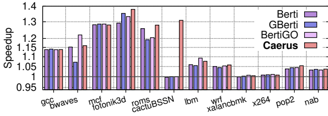
Fig. 15: Speedup of Caerus, Berti, GBerti, and BertiGO in SPECspeed 2017 workloads that show a performance delta of larger than 1%. Caerus outperforms BertiGO, the highest-performance, largest, most aggressive Berti variant, by 1.5% in the full SPECspeed 2017 suite (Fig. 1) and up to 30% in individual workloads.
