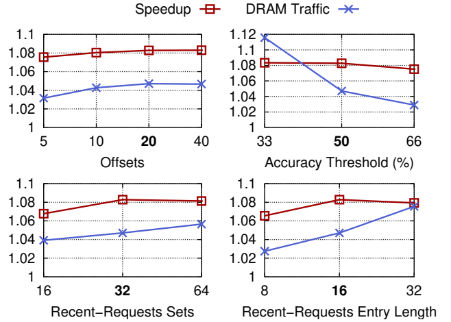
Fig. 20: Sensitivity study of Caerus parameters on SPECspeed 2017 (default parameters indicated in bold ).
