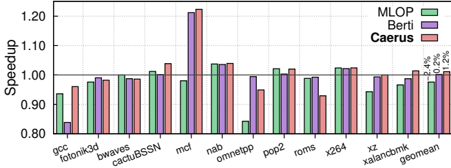
Fig. 19: Speedup of Caerus, MLOP, and Berti in 8-core SPECspeed 2017 homogeneous workloads that show a performance delta of larger than 1%.
