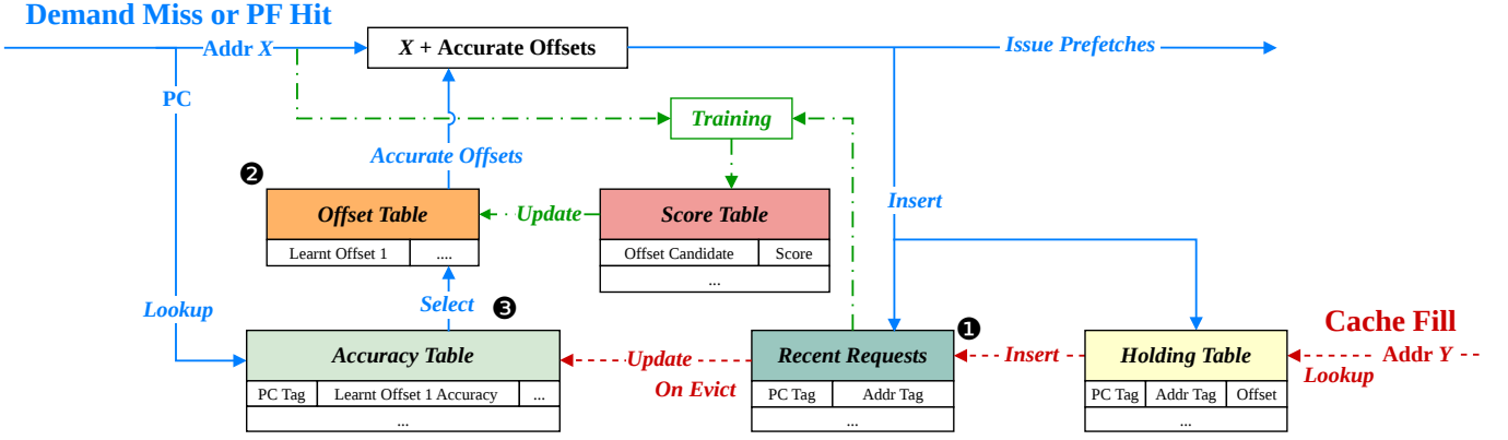
Fig. 6: Design of Caerus. On a demand miss/prefetch tag hit (solid blue), Caerus generates accurate offsets for prefetching (Section III-C). The accessed address is inserted into the Holding Table or Recent Requests (RR) Table (Section III-D). The Score Table is updated if deltas between the access and entries in the RR Table match an offset candidate (dot-dashed green) (Section III-A). Upon a cache fill (dashed red), matching Holding-Table entries update the RR Table (Sections III-C and III-D). Illustrations are given for ❶ RR-Table operations (Fig. 8), ❷ offset retraining (Fig. 9), and ❸ accurate offset selection (Fig. 10).
