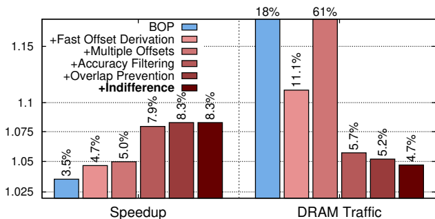
Fig. 21: Ablation Study. Starting with BOP and progressively adding Caerus’ features on SPECspeed 2017.
