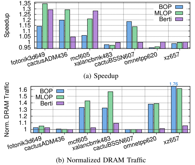
Fig. 4: Speedup and DRAM traffic of BOP, MLOP, and Berti in a selection of SPEC benchmarks.
