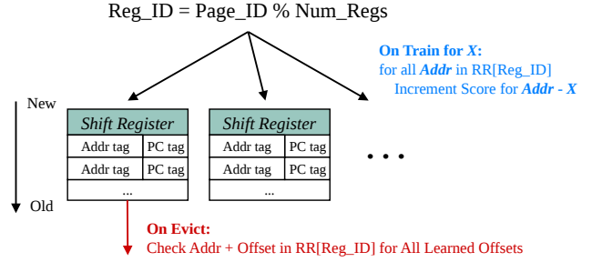
Fig. 8: Illustration of the operations on the Recent Requests (RR) table. When training a new address X , the scores of the deltas between X and the entries in the shift register with the same Reg_ID are incremented. When a shift register is full, each new insertion evicts the oldest entry (FIFO) and updates the accuracy of the learned offsets.
