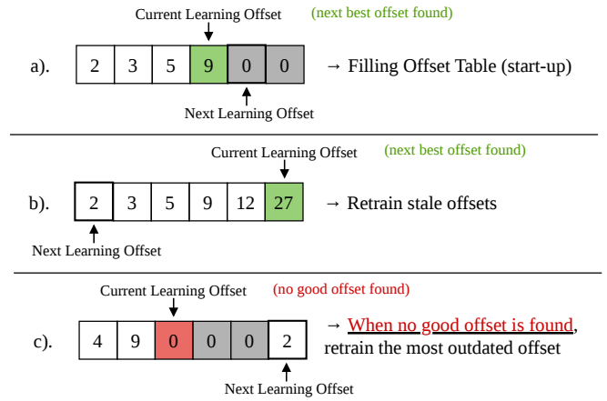
Fig. 9: Illustration of cyclical retraining. The Offset List is first filled with next best offset candidates (see Section III-A1). Caerus then continuously retrains its most outdated offsets to reflect changes in the memory access pattern.
