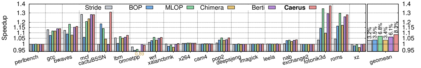
Fig. 11: Speedup on SPECspeed 2017: Caerus outperforms other techniques overall by succeeding in both PC-local and global prefetching settings, while avoiding contention from excess DRAM traffic harming performance.
