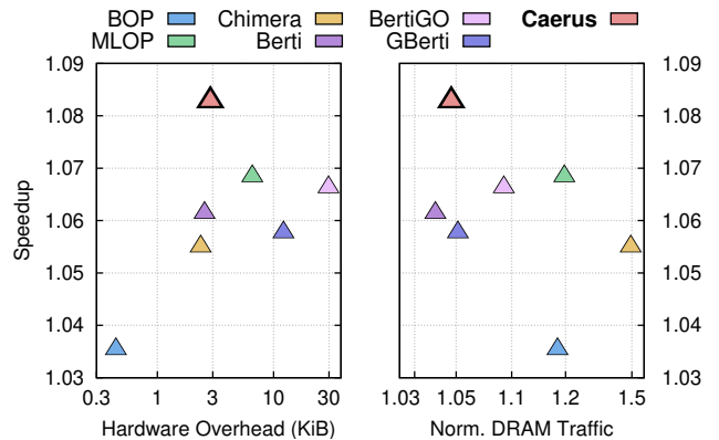
Fig. 1: Geomean speedup (SPEC2017) vs. hardware/DRAM-traffic overhead (log-scale) of BOP [19], MLOP [33], Chimera [14], Berti [25], BertiGO [35], GBerti [30] and Caerus. Caerus achieves the highest performance while incurring low DRAM traffic and hardware cost.
