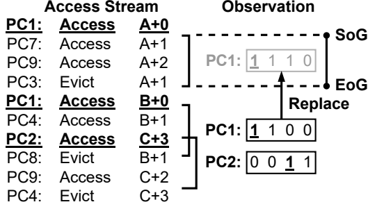
Figure 2: Basic operation of the Spatial Memory Streaming (SMS) prefetcher. SMS records the access pattern observed from the first access to a memory region until its first eviction, and reuses the recorded pattern to predict accesses when the same trigger feature is observed in another region.
