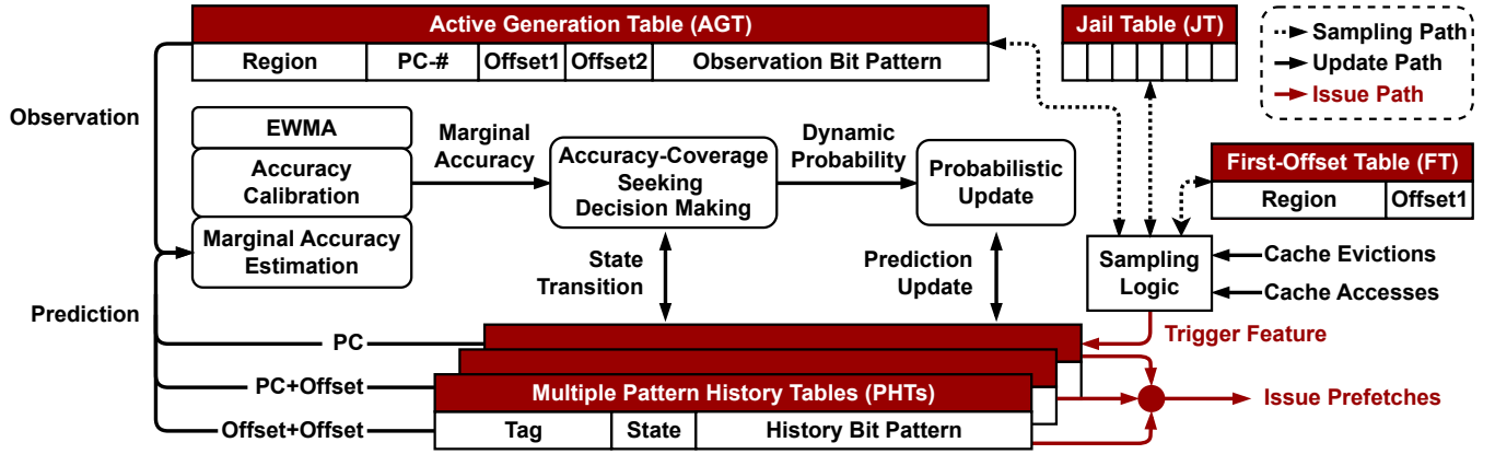
Figure 6: Design overview of Proba. Proba uses probabilistic updates to maintain accurate, high-coverage patterns in its Pattern History Tables (PHTs). Marginal accuracy dynamically controls prefetch aggression, while region sampling and Bloom-like hash-based mappings provide precise observation of cache-region generation behavior.
