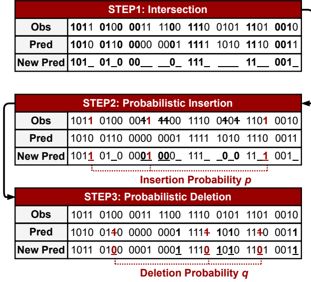
Figure 7: Probabilistic update of the Pattern History Table (PHT). Step 1 retains the intersection between the new observation (from the AGT) and the previous prediction (from the PHT). Step 2 inserts bits present in the observation but absent in the old prediction with an insertion probability p . Step 3 deletes bits present in the old prediction but missing in the new observation with a deletion probability q .
