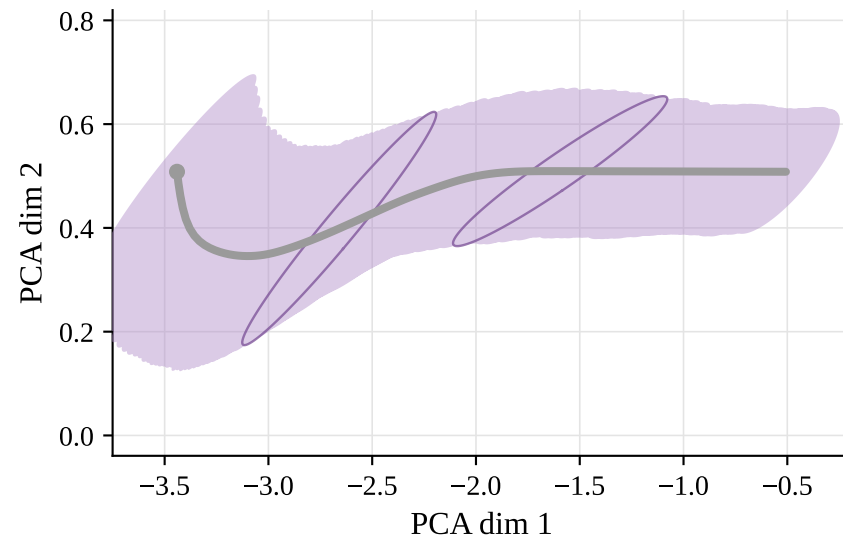
(a) Open-loop sampling \hat{\Sigma}_t
