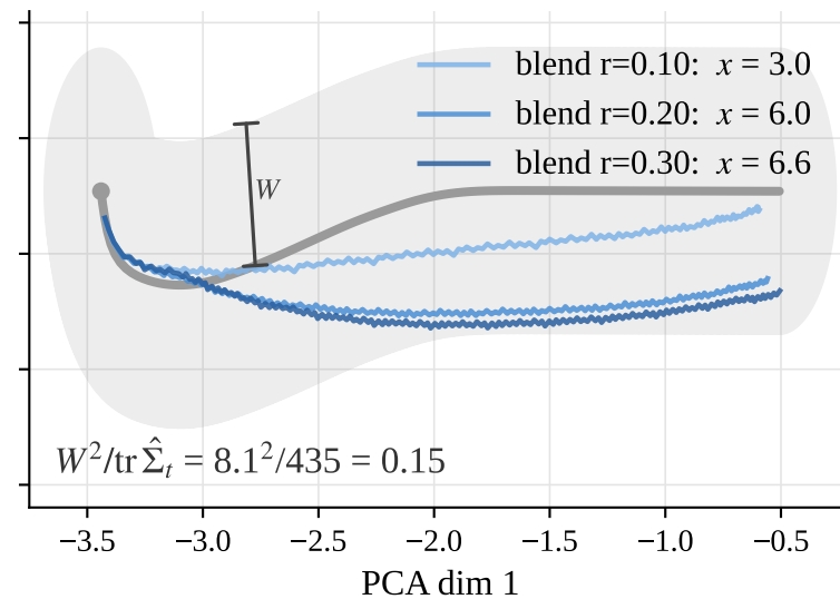
(b) Blend-guided rollouts settle at W
