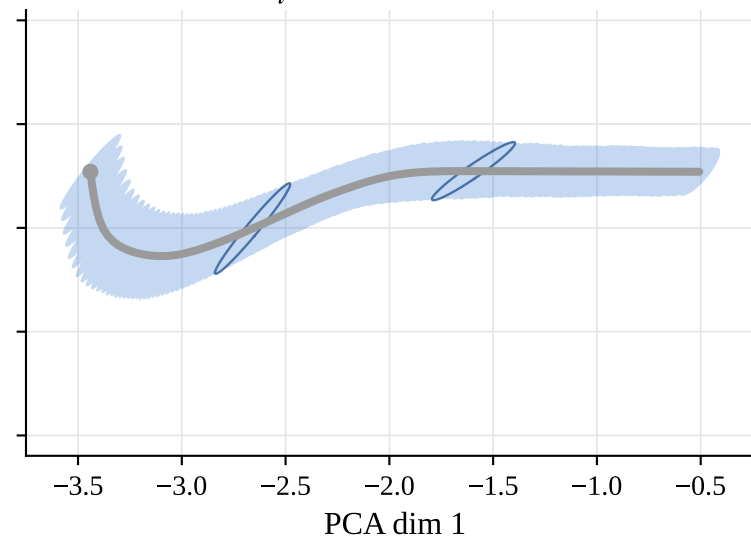
(c) Per-anchor \Sigma_t^\alpha = (W^2/\text{tr } \hat{\Sigma}_t) \hat{\Sigma}_t
