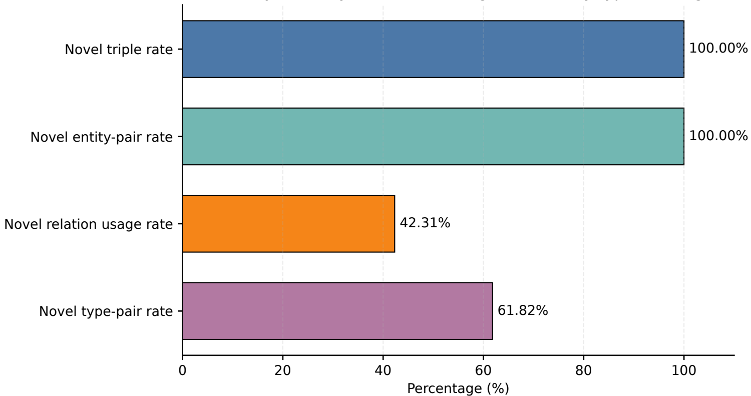
Novelty of Newly Added Knowledge After Entity-Type Filtering
