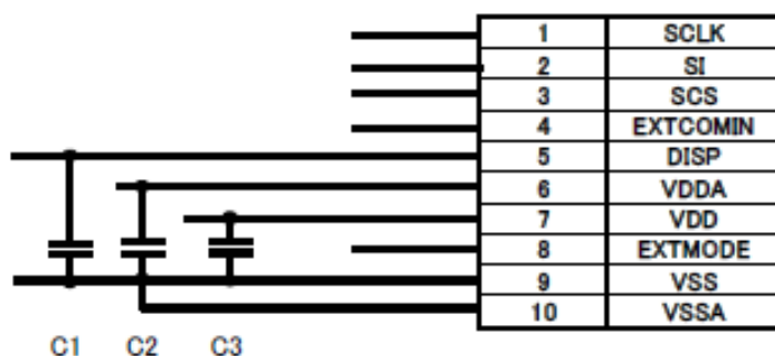
Figure 9-1 External Circuit (Recommended)
