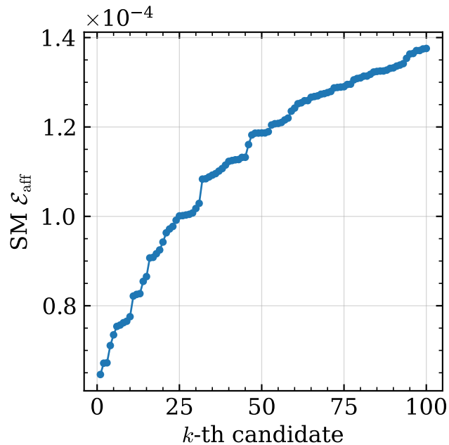
Top k candidate evaluation on kMC ground truth
