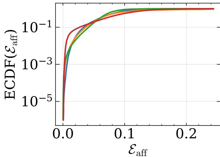
ReLU
